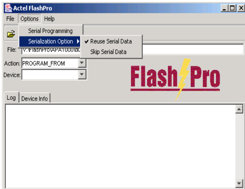
Figure 4-32. Serialization Option
