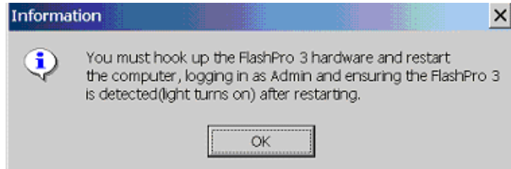
Figure 1-5. Information Box
