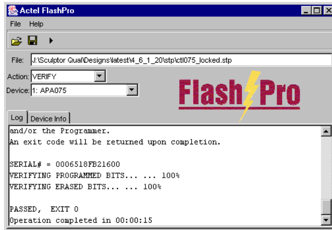
Figure 3-9. Successful Verification
