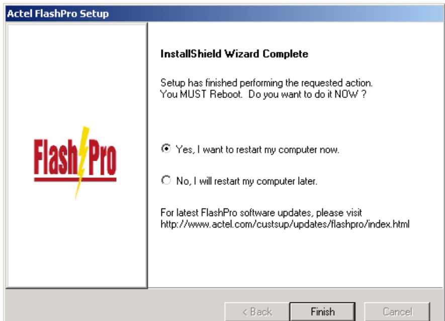
Figure 1-6. Installation Complete
