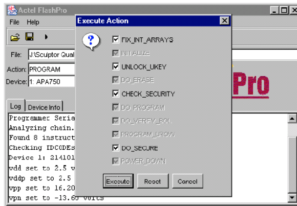
Figure 2-22. UNLOCK_UKEY Default
