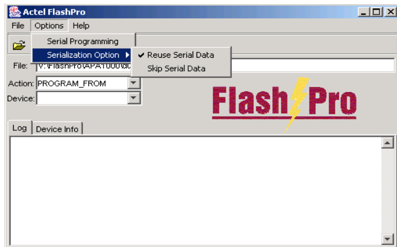
Figure 4-27. Serialization Option
