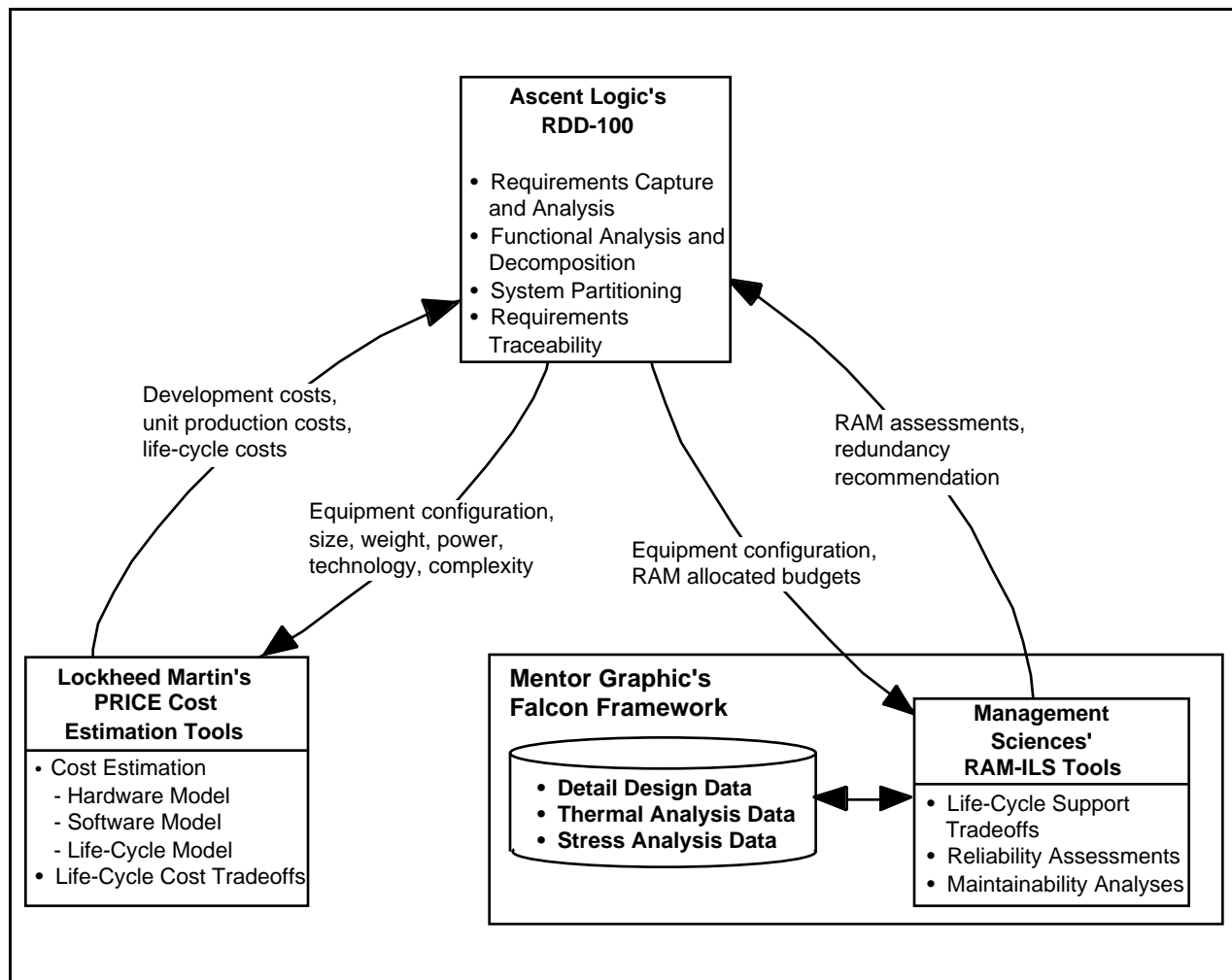
Figure 2.3-1. RDD-100/PRICE/RAM-ILS integration.
