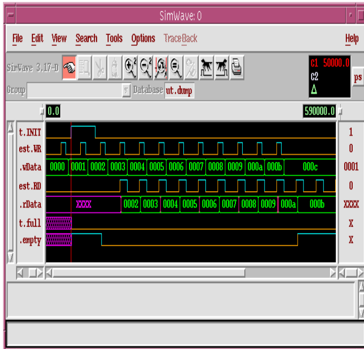
Figure 3-3. Edge-triggered FIFO
